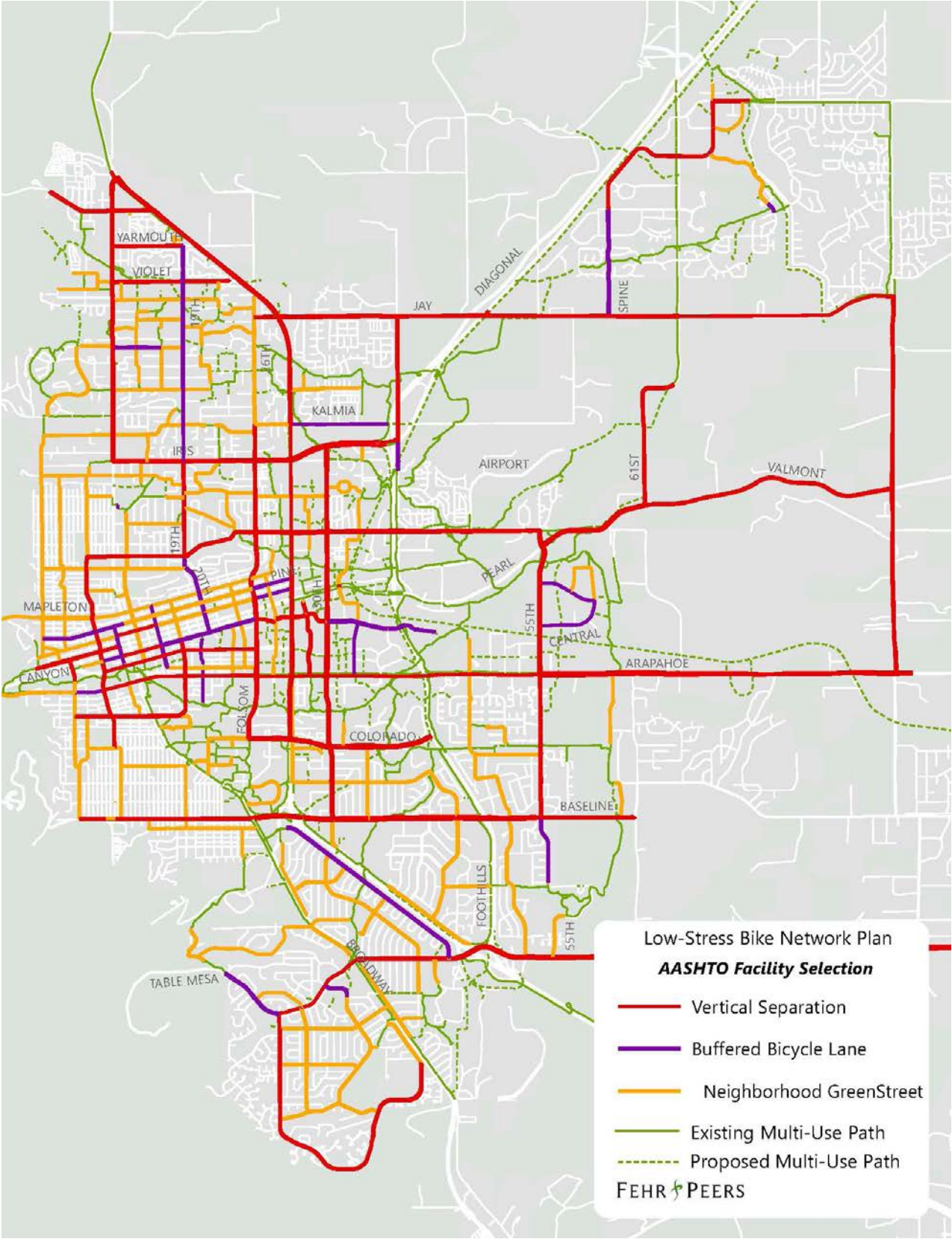
Figure 25. AASHTO Facility Type Selection
